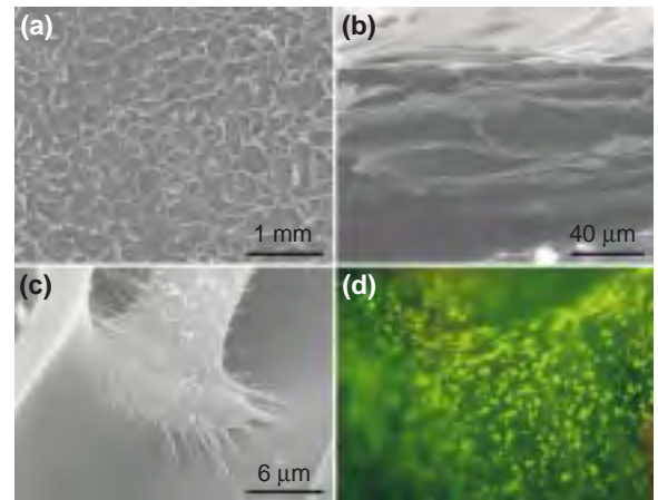
Fig. 1. Scanning electron micrographs of freeze-dried chitosan-gelatin scaffolds showing (a) Surface showing highly porous surface (scale bar = 1 mm). (b) Cross sectional view of scaffold showing extensive interconnections (scale bar = 40 \mu m). (c) Micrographs showing a human nasal septal chondrocyte establishing contact with scaffold matrix (scale bar = 6 \mu m). (Adapted from [11], Reproduced, with permission, from Cognizant Communication Corporation, NY, USA). (d) Cell viability evaluation in engineered cartilage construct. Human chondrocytes growing in fibre fleece scaffolds. Viable cells are labelled green by fluorescein diacetate.
