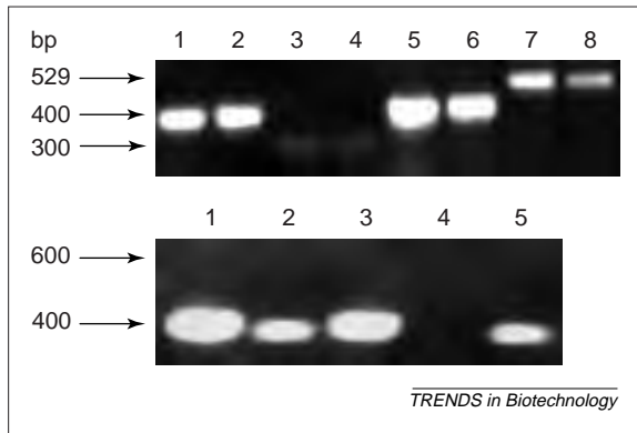
Fig. 2. Expression of various extracellular matrix proteins by chondrocytes growing on hydrogel scaffolds. (a) Gel picture shows the expression of Collagen Type II (COL II), aggrecan and COL IX obtained from two independent experiments. Hypoxanthine phosphoribosyltransferase (HPRT) was used as loading control to compare expression obtained from different experiments. Lane 1, 2 HPRT, Lane 3, 4 aggrecan, Lane 5, 6 COL II, Lane 7, 8 COL IX. Lane 1, 3, 5, 7: Experiment I and Lane 2, 4, 6, 8: Experiment II. (b) Comparative expression of COL I, COL II and COL III. Lane 1, 2, 3, 4 and 5 represents HPRT, COL I, COL II, COL X and COL III, respectively. Note higher expression ( p < 0.05 ) of COL II in comparison to COL I and III. Expression of COL X could not be detected. (Adapted from [13] and reproduced, with permission, from Cognizant Communication Corporation, NY, USA)
